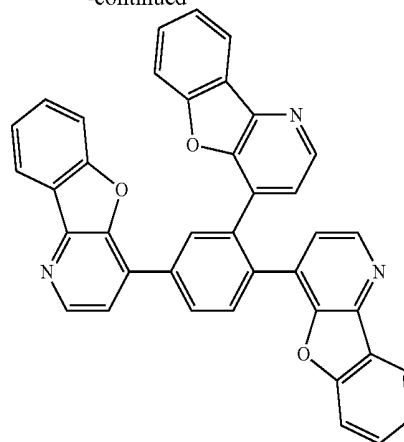
Example compound M-197
